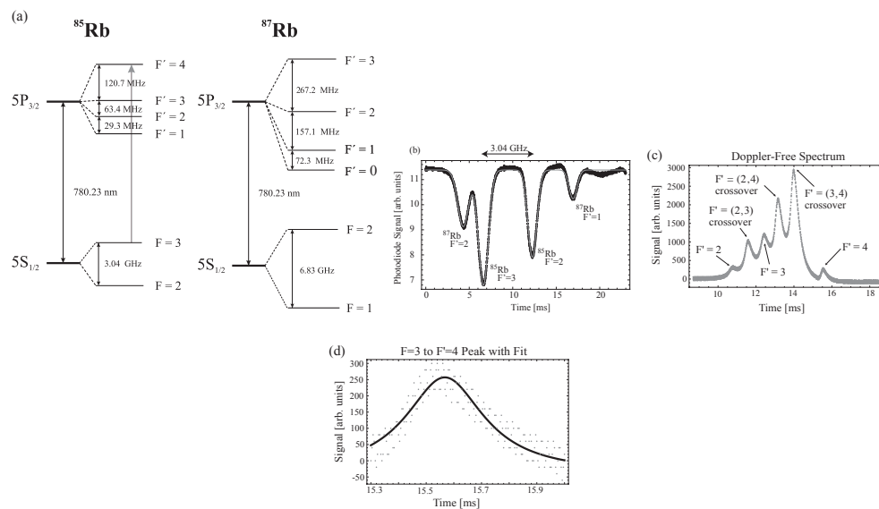
Figure 2. (a) Energy level diagrams for 85 Rb and 87 Rb. The Rb reference cell contains the two naturally occurring isotopes in the number ratio of 72:28. (b) Oscilloscope trace of Doppler broadened absorption spectra in 85 Rb and 87 Rb observed by scanning the external cavity diode laser (ECDL). The ground states corresponding to each peak are labeled. The frequency interval between the two ground states in 85 Rb is marked. The time axis can be converted to frequency units based on the known separation between energy levels. The full width at half maximum (FWHM) extracted from a Gaussian fit of the F = 3 \rightarrow F' = 2, 3, 4 resonance is 735 \pm 5 MHz. Based on Beer’s law, I = I_0 e^{-\alpha(\nu)l} where \alpha(\nu) is the absorption coefficient, l is the length of the Rb cell, I_0 is the incident intensity and I is the transmitted intensity. We find that the maximum absorption corresponds to an optical depth of \alpha_0 l = 0.516 \pm 0.003 , where \alpha_0 = \alpha(\nu_0) and \nu_0 is the resonance frequency. (c) Oscilloscope trace of Doppler-free spectrum for the 85 Rb F = 3 \rightarrow F' = 2, 3, 4 transitions. The frequency interval between the F' = 4 peak and the adjacent crossover resonance is 60.4 MHz. (d) An expanded plot of the F = 3 \rightarrow F' = 4 resonance line. A FWHM of 12.7 \pm 0.9 MHz is obtained from a Lorentzian fit. In general, this value should have contributions from the natural broadening ( \sim 6 MHz), power broadening, and laser linewidth.
