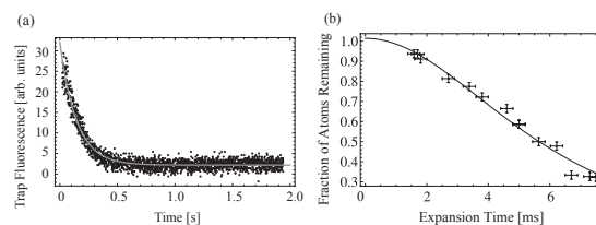
Figure 27. (a) Measurement of the optical molasses decay time. A fit to a decaying exponential gives a 1/e time constant of 0.165 \pm 0.002 s. (b) Measurement of the temperature of trapped atoms using the release and re-capture method. The vertical axis represents the fraction of re-captured atoms. The horizontal axis is the free expansion time. A determination of the most probable speed u from the fit gives a temperature T = 420 \pm 20 \mu K.
