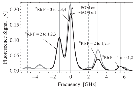
Figure 4. Fluorescence spectra from a pump laser beam passing through an EOM and a Rb vapor cell. The laser is scanned over several GHz and a fluorescence signal is recorded by photodiode C in Figure 3. The black curve shows the fluorescence with the EOM off. The grey curve is obtained with the EOM on. The operating frequency of the EOM is 2.915 GHz which represents the energy difference between the F = 3 \rightarrow F' = 4 and F = 2 \rightarrow F' = 3 transitions in ^{85}\text{Rb} .
