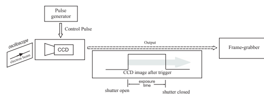
Figure 13. A charged coupled device (CCD) camera and frame grabber are used to measure the fluorescence of an electron beam as it sweeps across the screen of an analog oscilloscope. A pulse generator is used to generate a TTL pulse that controls the shutter of the CCD camera.
