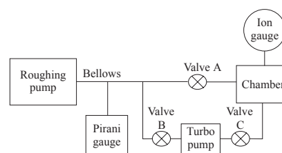
Figure 16. Vacuum system used in the experiment. In the first stage of the experiment, valves B and C are closed and the chamber is pumped directly using the roughing pump. In the second stage, valve A is closed and the chamber is pumped by the turbo pump in series with the roughing pump.
