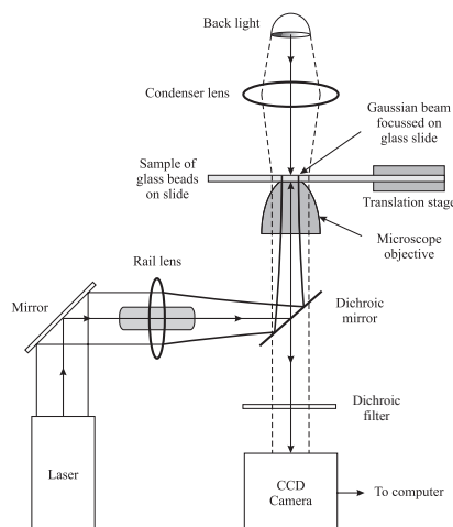
Figure 17. Schematic diagram of the optical tweezers experiment. The laser source is a diode laser operating at \lambda = 532\ \text{nm} . The dichroic mirror ensures that most of the laser light reaches the microscope objective. The rail lens is used to vary the size of the laser beam. The objective focuses the laser beam to a spot size of \sim 3\ \mu\text{m} . The sample of polystyrene glass beads in saline solution is placed at the focal spot of the laser. The sample is uniformly illuminated by a backlight. Light from this lamp source passes through a condenser lens and the sample. After passing through the microscope objective, it is imaged on a CCD camera. With the laser blocked, the CCD camera can image the glass beads suspended in solution. When the optical dipole force trap is aligned, the dichroic mirror and dichroic filter ensure that a small fraction of the light scattered by the trapped beads reaches the CCD camera. The scattered light follows the same optical beam path as the backlight and is sufficiently intense for the trapped bead to be imaged.
