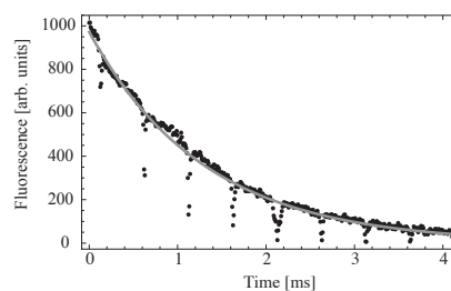
Figure 14. Intensity of fluorescence due to an electron beam sweeping across the screen of a line triggered oscilloscope recorded by a shutter-controlled CCD camera. The dips in intensity correspond to the grid lines on the oscilloscope. The spacing between the grid lines is determined by the time base setting of the oscilloscope, thereby allowing the pixel axis to be converted to a time scale. The solid curve is the best fit to the data based on a decaying exponential. The fit gives a decay time of 1.30 \pm 0.03 ms.
