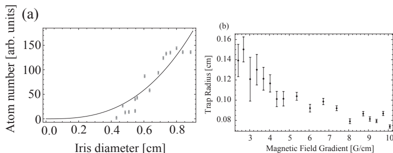
Figure 24. (a) Atom number as a function of iris diameter, d . The data shows a sensitive dependence on the beam size. For a well aligned trap and a well centered iris, the atom number can be expected exhibit a power law dependence shown by the solid line. For this experiment, the trap detuning was set to 15 MHz below resonance, the trap laser power was \sim 65 mW, the repump laser power was set at \sim 15 mW, and the magnetic field gradient was \sim 7 G/cm. (b) Cloud radius ( 1/e ) as a function of magnetic field gradient along the vertical direction. For this data, the trap laser power was fixed at \sim 75 mW and the trap laser detuning was \sim 15 MHz below resonance with a beam diameter of \sim 1.0 cm. The repump power was \sim 12 mW.
