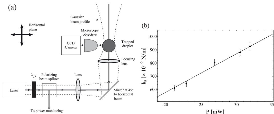
Figure 20. (a) Modified experimental set-up for free-space trapping experiment. (b) Spring constant of the trap as a function of laser power for a charcoal particle confined in free-space. The horizontal axis has been corrected for the power loss of the microscope objective.
