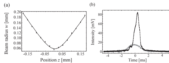
Figure 15. (a) Beam radius, w , orthogonal to the direction of propagation as a function of distance ( z ) from a 20 cm focal length plano-convex lens. The beam size was measured using a scanning knife edge beam profiler. The position z = 0 represents the focal spot. The solid line is a fit to the equation w = w_0[1 + (z - z_1)^2/z_0^2]^{1/2} , where z_0 = \pi w_0^2/\lambda . Here, w_0 is the minimum beam radius, z_0 is the Rayleigh range and z_1 is an offset that specifies the location of the minimum beam radius from the origin. The fit gives w_0 = (58.7 \pm 1.3) \mu\text{m} , z_0 = (5.8 \pm 0.2) \text{cm} , and z_1 = (4.6 \pm 0.8) \text{mm} . (b) Spatial profile of a laser beam before (black) and after (grey) passing through an optical fiber. The profile at the entrance to the fiber was obtained by distorting the beam using a scratched cover slide. The profiles represent the analog outputs of a scanning knife edge spatial profiler.
