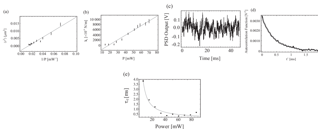
Figure 19. (a) Mean squared displacement as a function of inverse laser power. The power represents the measured value at the entrance to the microscope objective. Only ~50% of the light reaches the sample. (b) Spring constant of the dipole force trap as a function of laser power. The horizontal axis has not been corrected for the power loss at the microscope objective. The points representing the spring constant are calculated from the data in (a) on the basis of the equipartition theorem. (c) Signal from the position sensitive detector (PSD), which represents the position of the bead as a function of time. (d) Autocorrelation function (black) calculated from the PSD signal by fitting to a Lorentzian (grey) for a small section of the data such as in figure (c). The horizontal axis represents the time lag between the data points in the record. The fit gives a correlation time \tau_c = 0.422 \pm 0.005 ms. (e) Correlation time as a function of laser power.
