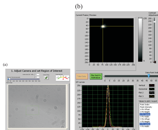
Figure 18. (Color online) Display of the LabVIEW interface used to record and analyze CCD images of the trapped beads. (a) Image of beads suspended in solution. (b) The upper frame shows the image of a 2 μm diameter trapped bead. The corresponding intensity profile is displayed in the lower frame.
