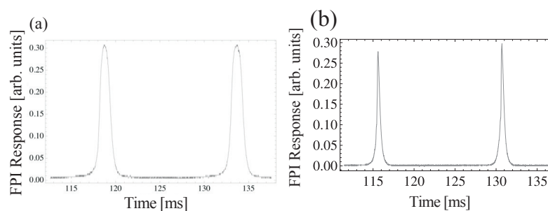
Figure 7. Transmission peaks obtained by operating the diode laser at a fixed frequency and scanning the Fabry-Pérot interferometer (FPI). (a) FPI peaks without grating feedback. The measured FWHM is 133 \pm 5 MHz. (b) FPI peaks with grating feedback. The measured FWHM of 67 \pm 3 MHz is comparable to the calculated resolution of the FPI. The value of the free spectral range of the spherical mirror FPI ( c/4L ), calculated on the basis of the known cavity length of L = 7.5 cm is \sim 1 GHz. Since the separation between adjacent transmission peaks is equal to the free spectral range, it is possible to convert the time axis into frequency units.
