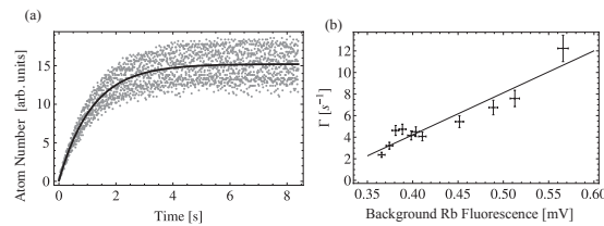
Figure 26. (a) Loading curve for the magneto-optical trap (MOT). The data was recorded for a fixed n_{\text{Rb}} . A fit to the functional form described in text gives \Gamma^{-1} = 1.17 \pm 0.03 \text{ s} . (b) Variation of the collisional rate with background fluorescence, which is proportional to n_{\text{Rb}} .
