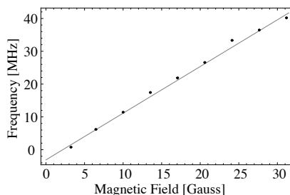
Figure 5. The frequency shift of the F = 3 \rightarrow F' = 4 transition as a function of magnetic field. The frequency shift is obtained by recording the position of the spectral line in a Rb cell placed in a magnetic field relative to the position of the spectral line without a magnetic field. A value of 1.49 \pm 0.08 MHz/G for the Zeeman shift is found from the slope of a straight line fit. The expected value for the Zeeman shift of the m_F = 3 \rightarrow m_{F'} = 4 sublevel transition is 1.4 MHz/G. The horizontal error bars are estimated to be \pm 5\% and the vertical error bars are comparable to the size of the points.
