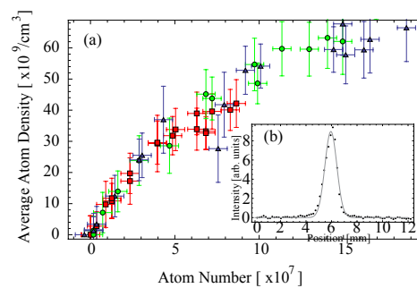
Figure 23. (Color online) (a) Variation in average density as a function of atom number. The atom number, inferred from trap fluorescence, was varied by changing the trap laser power. The trap laser detuning was fixed at 15 MHz below resonance, the trapping beam diameter was \sim 0.90 cm and the magnetic field gradient was \sim 7 G/cm. Three different repump laser powers were used, 0.60 \pm 0.06 mW (red squares), 1.0 \pm 0.1 mW (green circles), and 50 \pm 5 mW (blue triangles). The cloud radius was determined from fits along two dimensions that were summed in quadrature. (b) Spatial profile of the cloud obtained from a CCD camera image for a trap laser power of 75 \pm 7 mW, repump laser power of 50 \pm 5 mW, and a magnetic field gradient of \sim 7 G/cm. The vertical axis represents the intensity obtained by integrating pixel values. A Gaussian fit gives a 1/e^2 cloud radius of 0.66 \pm 0.01 mm.
