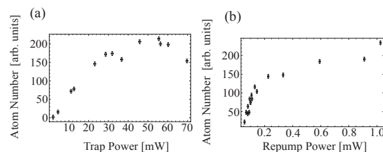
Figure 22. (a) Steady state atom number as a function of trap laser power. The atom number is inferred by recording the trap fluorescence on a photodiode. The voltage recorded by the detector can be converted into atom number. The maximum voltage corresponds to an atom number of \sim 10^7 . Since the trap laser is retro-reflected through the vacuum chamber, the laser power incident on the atoms is approximately twice the trap laser power. (b) Atom number as a function of repump laser power. For both of these experiments, the trap laser detuning was fixed at 15 MHz below resonance, the trapping beam diameter was \sim 0.90 \text{ cm} and the magnetic field gradient was \sim 7 \text{ G/cm} .
