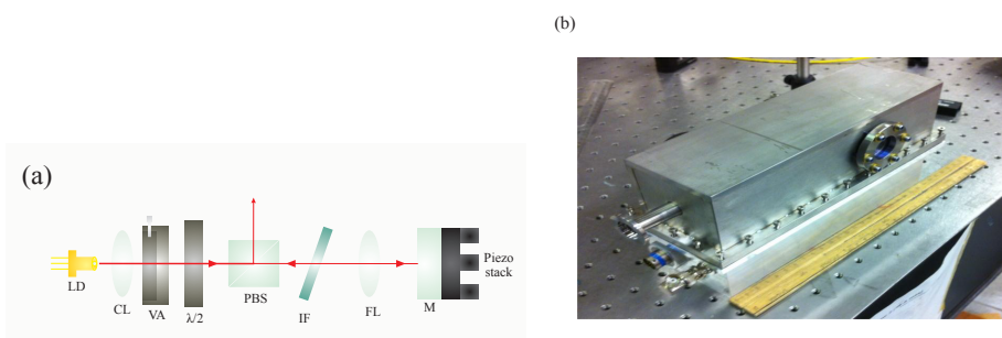
Figure 1. (a) Layout of IF laser. The optical elements are: LD—laser diode, CL—collimating lens, VA—variable aperture, \lambda/2 —half wave-plate, PBS—polarizing beam splitter, IF—interference filter, FL—focusing lens, M—mirror. (b) Home-built IF-laser head.
