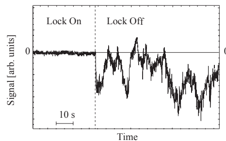
Figure 11. Lock-in error signal recorded with and without engaging the feedback loop. For both parts of the trace, the scan amplitude has been turned off, whereas the modulation remains on. The amplitude variations are mainly due to laser frequency fluctuations, which are greatly reduced with the feedback loop engaged (lock on). Under typical operating conditions, the diode laser remains locked for about 30 min.
