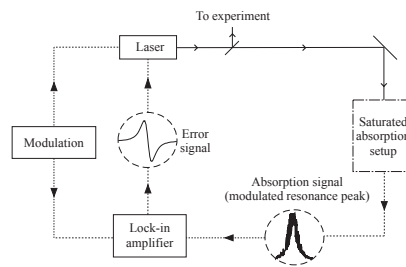
Figure 8. Setup for laser frequency stabilization using a lock-in amplifier. The modulation was provided by a function generator operating at \sim 7 kHz. A scan controller is used to scan the laser frequency at a rate of \sim 10 Hz. An example of the saturated absorption setup is shown in Figure 3. A trace of the saturated absorption signal obtained by scanning the laser over a single Doppler-free transition is shown. For illustrative purposes, this trace was recorded with a large amplitude for frequency modulation. The output of the lock-in amplifier generates the corresponding dispersion shaped error signal. To lock the laser to the peak of this resonance line, the laser frequency is centered on the resonance peak, and the scan amplitude is gradually reduced (ideally to zero) before engaging the feedback loop.
