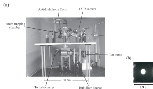
Figure 21. (a) A portion of the atom trapping setup. A pair of anti-Helmholtz coils is used to apply a magnetic field gradient. Two pairs of the trapping beams are aligned in the horizontal plane between the anti-Helmholtz coils. An orthogonal trapping beam is aligned along the vertical. (b) Image of trapped ^{85}\text{Rb} atoms recorded by a CCD camera. An optimized trap has a 1/e^2 cloud radius of \sim 1 mm and holds \sim 10^7 atoms. The CCD image of the trap in (b) is saturated causing blooming.
