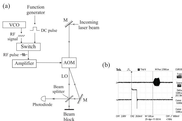
Figure 12. (a) Heterodyne detection setup. The incoming beam is generated by an ECDL operating at 780 nm. The optical local oscillator (LO) is the undiffracted beam from the acousto-optic modulator (AOM). Light from one of the ECDL-based experiments described previously is aligned through th. The first order diffracted beam from the AOM is rendered co-propagating with the LO using a beam splitter and mirrors so that a heterodyne beat signal can be detected by the photodiode. The RF input to the AOM is either CW or pulsed, and the control electronics are shown. The output of the TTL switch is an RF pulse that drives the AOM. (b) The square pulse used to amplitude-modulate the AOM and corresponding time-delayed optical pulse detected by the photodiode. The square pulse is the signal input to the electronic TTL switch, which also triggers the oscilloscope. The optical pulse exhibits a beat note at the AOM drive frequency. The time delay between the onset of the square pulse and the beginning of the optical pulse is 3.45 \pm 0.05 \mu\text{s} . This delay is consistent with the estimated time for an acoustic wave to propagate from the transducer at the edge of the AOM crystal to the location of the laser beam passing through the AOM.
