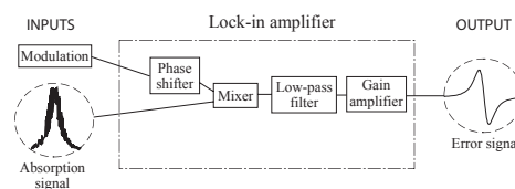
Figure 9. Schematic diagram showing the essential components of a lock-in amplifier.
