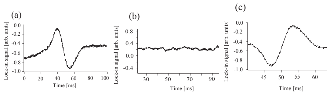
Figure 10. Lock-in output (error signal) obtained by scanning the laser across a resonance line for various phase shifts between the absorption signal and the modulation: (a) \phi = 0^\circ , (b) \phi = 90^\circ and (c) \phi = 180^\circ .
