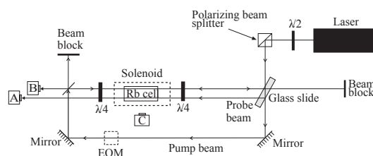
Figure 3. Saturated absorption setup used in emission and absorption spectroscopy, Zeeman shift, and laser frequency stabilization experiments. A quarter-wave plate represented by \lambda/4 is used to produce circularly polarized laser beams. A half-wave plate, represented by \lambda/2 , is used to control the ratio of power reflected and transmitted by the polarizing beam splitter. “A” and “B” represent photodiodes used for recording absorption spectra. The absorption of a weak probe beam that serves as a reference is recorded by photodiode A. The absorption of a weak probe beam in the presence of a strong counter-propagating pump beam is recorded by photodiode B. Electronic subtraction of the signals from these photodiodes gives a Doppler-free spectrum shown in Figure 2c. Photodiode C is used to record right-angle fluorescence. Locations of the electro-optic phase modulator (EOM) used in the emission and absorption spectroscopy experiment and the solenoid used in the Zeeman shift experiment are shown by dashed lines. In experiments with the EOM, the two weak probe beams are blocked and only the pump beam remains on.
