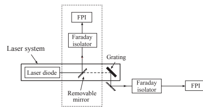
Figure 6. Experimental setup for measurement of the laser linewidth using a FPI. The grating in the ECDL cavity is bypassed by inserting a mirror attached to a removable mount so that the linewidth of the free running laser diode can be determined. This configuration is shown by the dotted box. When the mirror is removed, the linewidth of the laser is much smaller ( \sim 1 MHz) due to the presence of grating feedback. Since the FPI resolution is \sim 60 MHz, only the instrument limited linewidth is measured in this case.
